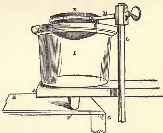
FIG. II. CROOKES' APPARATUS.
